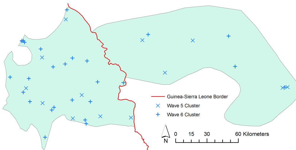
Figure 5: DHS Clusters Across Waves in the Kuranko Language Group Partition
